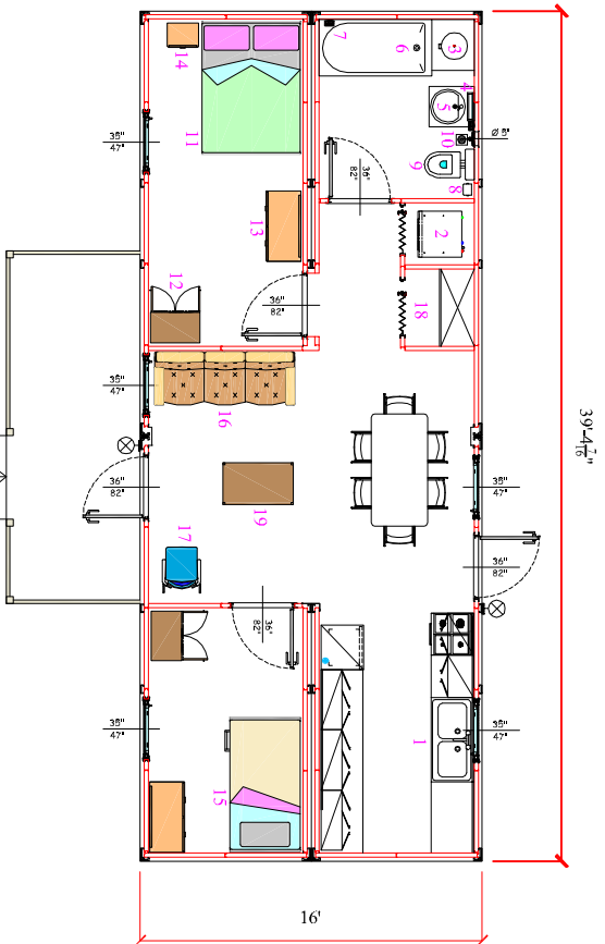
VIEW -B-
